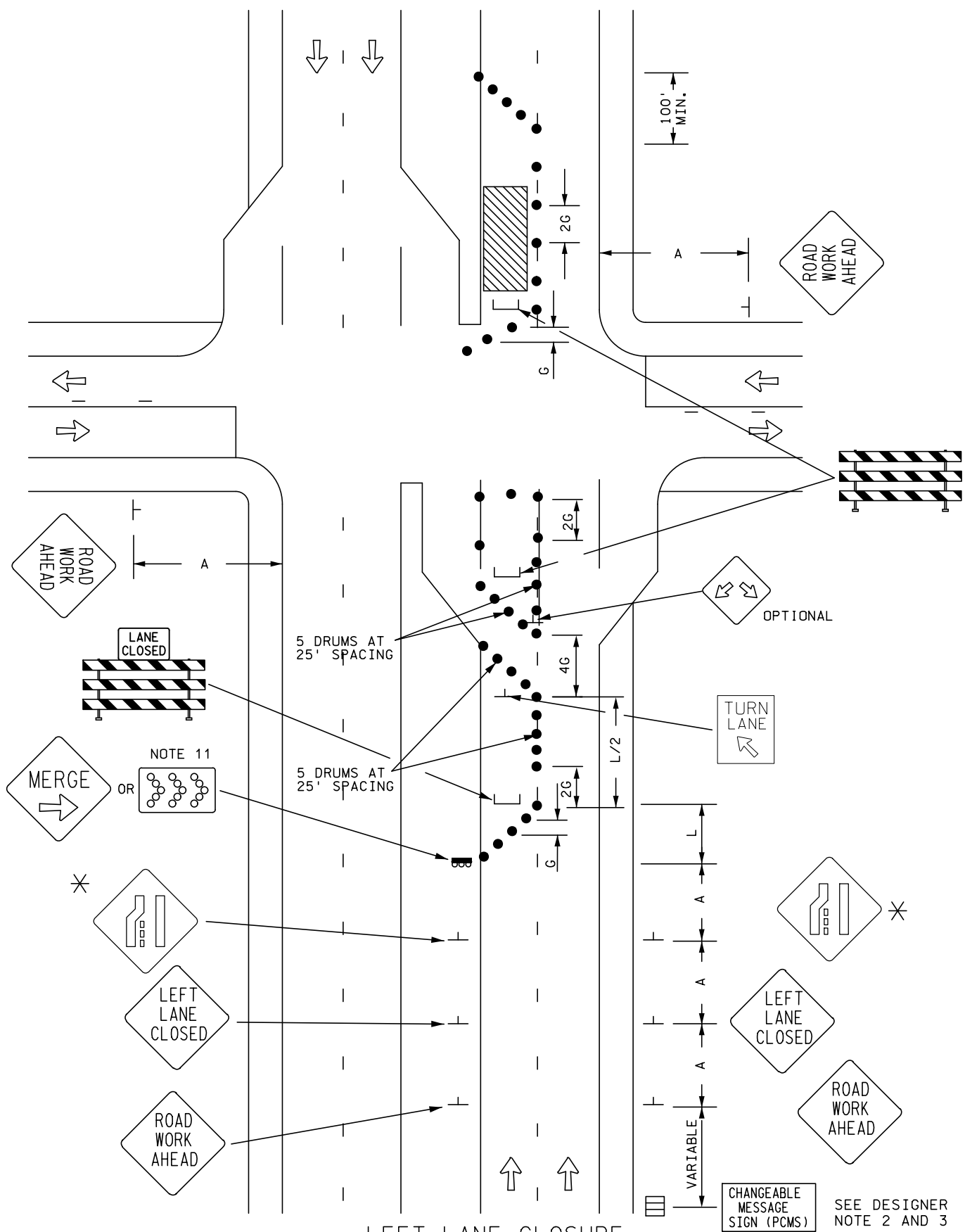
LEFT LANE CLOSURE WORK SPACE BEYOND INTERSECTION MULTI-LANE DIVIDED ROAD NOT TO BE USED FOR MORE THAN THREE CALENDAR DAYS
